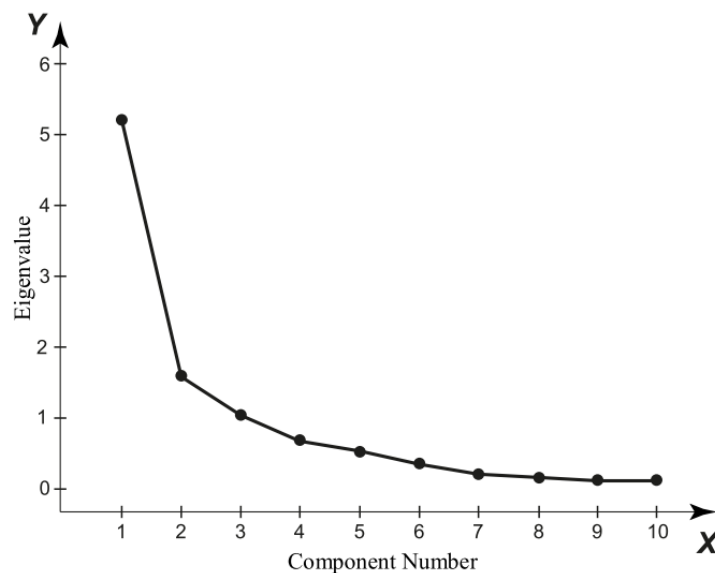
Figure 2. Initial Eigenvalues
